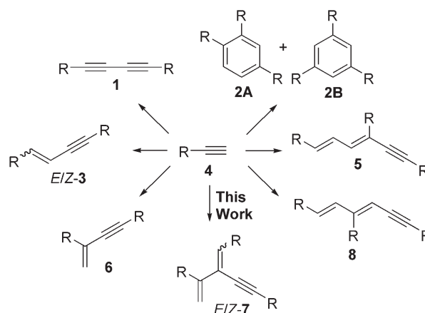
Scheme 1. Metal-catalyzed oligomerizations of terminal alkynes.
