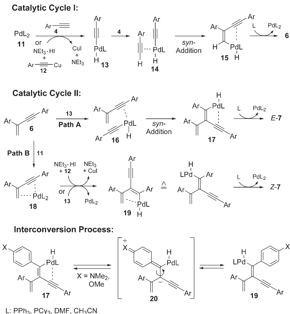
Scheme 2. Proposed mechanism for the formation of a dienyne 7 .
