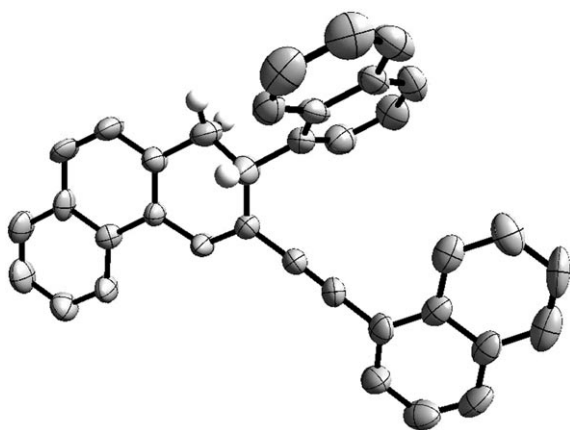
Figure 2. The molecular structure of 21 showing 50% probability ellipsoids (Diamond version 3.0). Hydrogen atoms except for 1- and 2-H have been omitted for clarity. [29]
