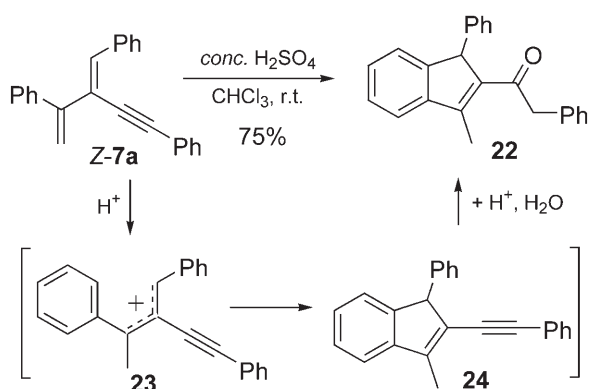
Scheme 3. Synthesis of indene 22 from dienyne Z - 7a in acidic conditions.
