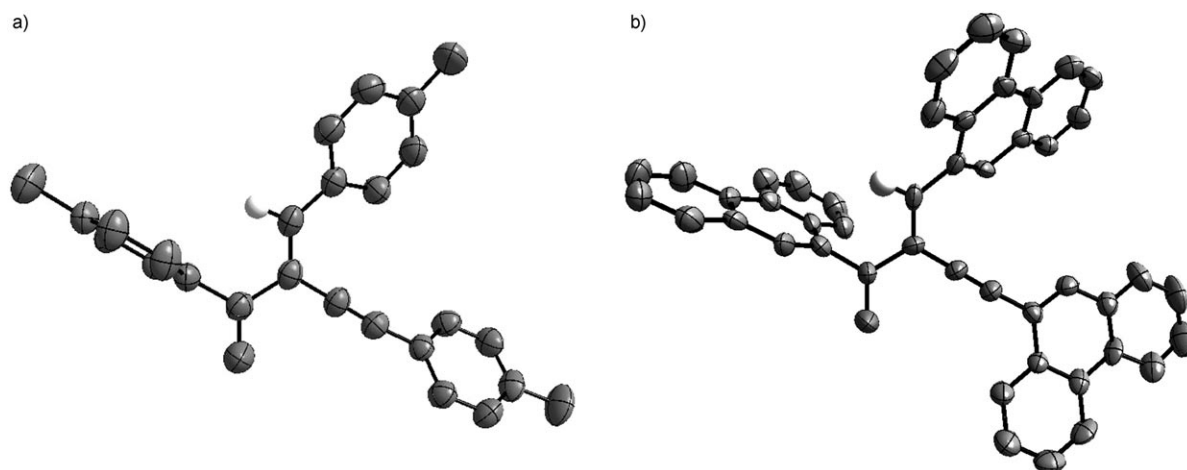
Figure 1. The molecular structures of Z-7d (left) and Z-7o (right) showing 50% probability ellipsoids (Diamond version 3.0). Hydrogen atoms except for 3-H have been omitted for clarity. [21]
